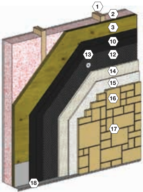
WOOD/STEEL FRAMING
