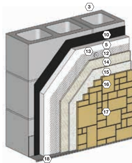
RIGID INSULATION ON CMU OR CONCRETE WALL SYSTEMS
