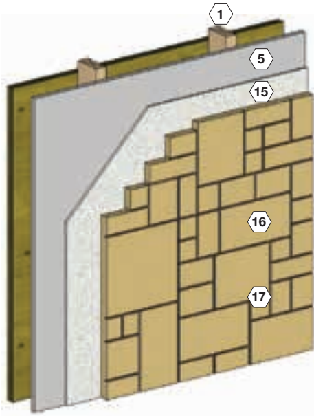
INTERIOR-CEMENT BOARD
