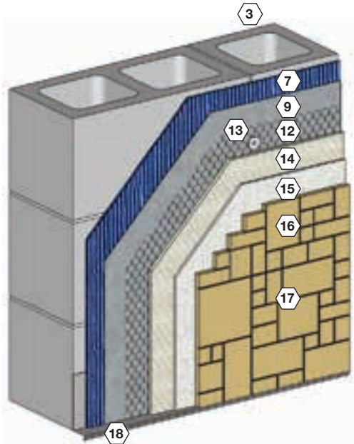
RIGID INSULATION WITH ADDITIONAL SHEATHING
